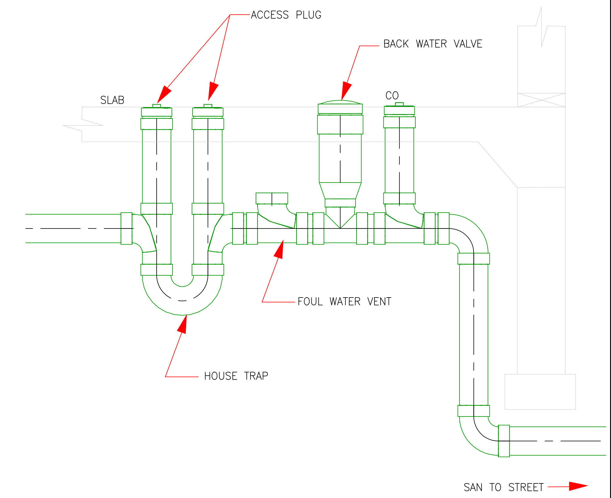
HOUSE TRAP DETAIL SCALE-NTS
