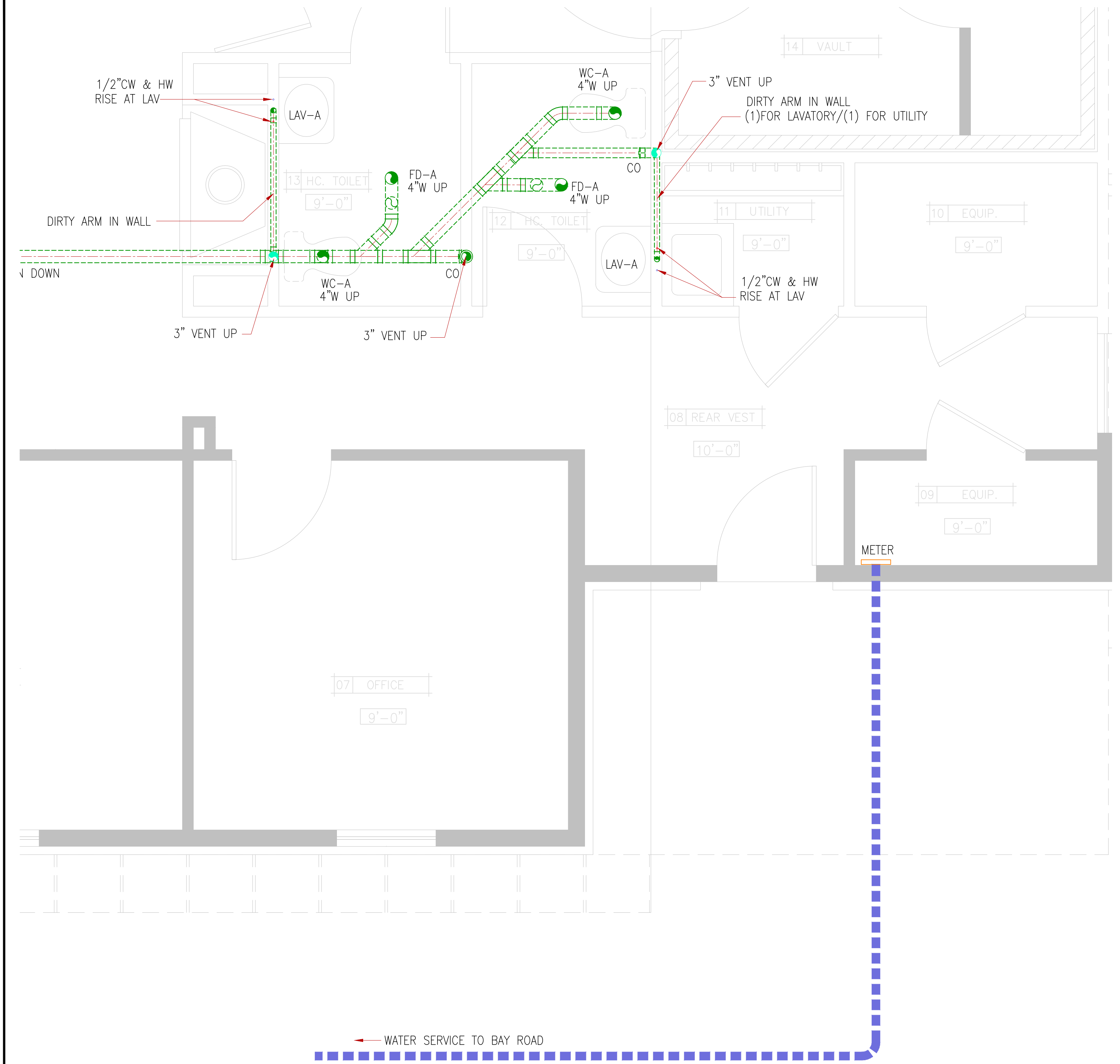
1 ENLARGED PLUMBING PLAN SCALE: 1/2"=1'
