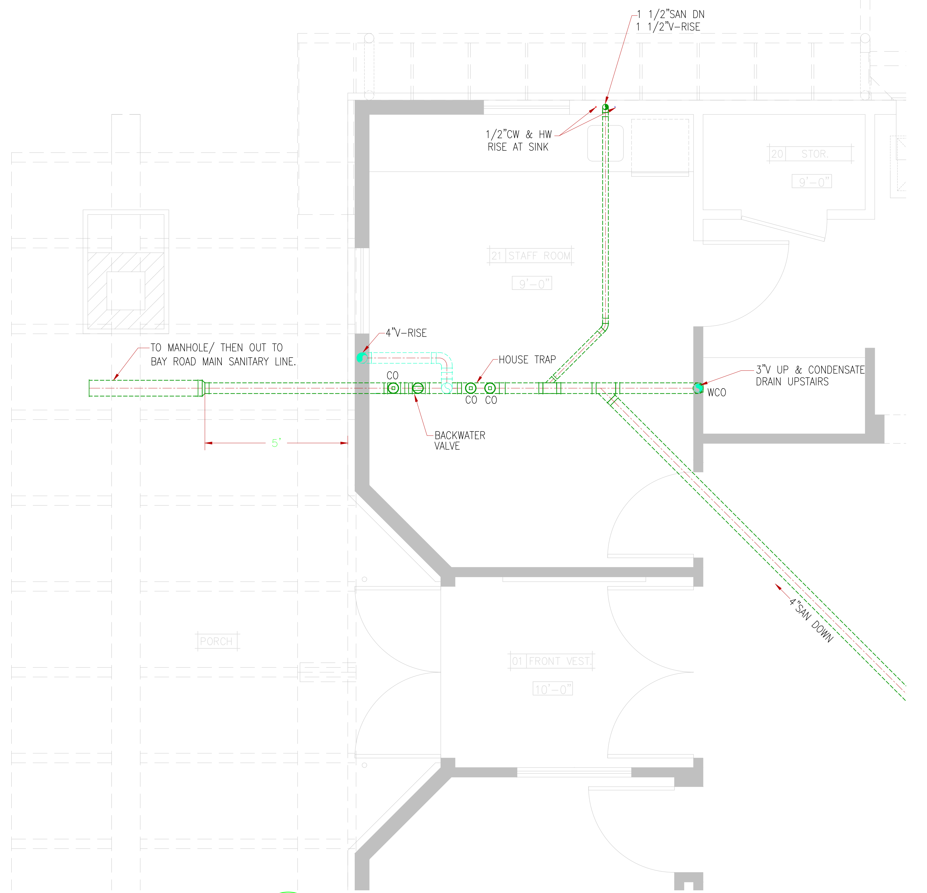
2 ENLARGED PLUMBING PLAN SCALE: 1/2"=1'
